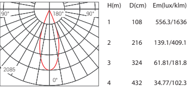
Beam Angle 38° 12W 3000K
