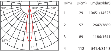
Beam Angle 12° 25W 3000K
