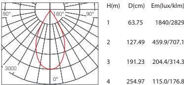
Beam Angle 40° 10W 3000K
