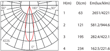
Beam Angle 24° 25W 3000K
