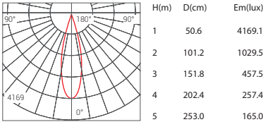
Beam Angle 24° 18W 3000K
