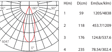
Beam Angle 38° 22W 3000K
