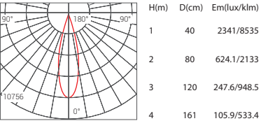
Beam Angle 24° 22W 3000K
