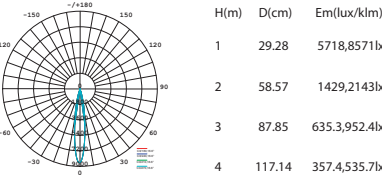
Beam Angle 16.6° 20W
