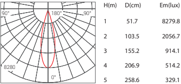
Beam Angle 24° 50W 3000K
