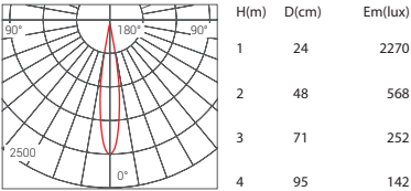
Beam Angle 15° 8W 3000K
