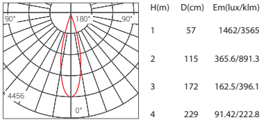
Beam Angle 24° 15W 3000K
