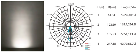
Beam Angle 34.4° 12W
