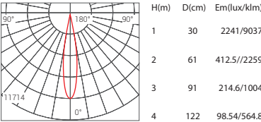
Beam Angle 12° 12W 3000K
