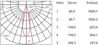
Beam Angle 24° 40W 3000K
