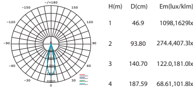
Beam Angle 26.4° 6W
