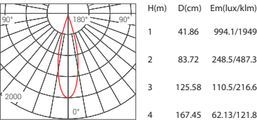
Beam Angle 20° 10W 3000K
