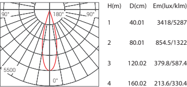
Beam Angle 20° 15W 3000K
