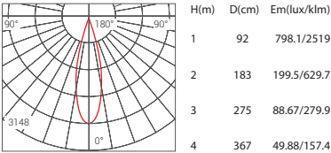
Beam Angle 24° 10W 3000K
