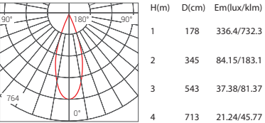
Beam Angle 120° 30W 3000K
