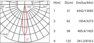
Beam Angle 15° 22W 3000K
