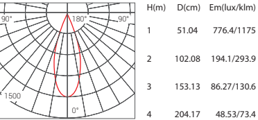
Beam Angle 38° 6W 3000K
