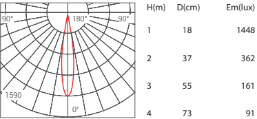
Beam Angle 15° 3W 3000K
