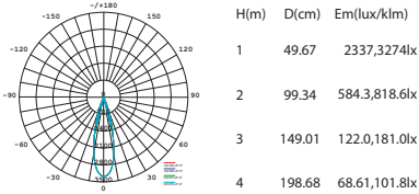
Beam Angle 27.9° 12W
