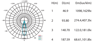
Beam Angle 26.4° 6W
