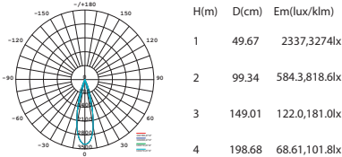
Beam Angle 27.9° 12W
