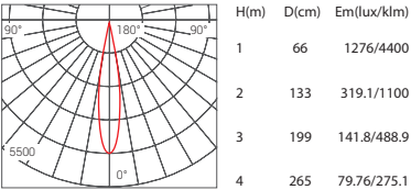
Beam Angle 15° 10W 3000K
