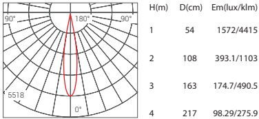
Beam Angle 15° 15W 3000K
