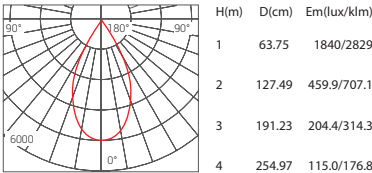
Beam Angle 40° 15W 3000K
