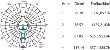
Beam Angle 16.6° 20W
