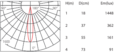
Beam Angle 15° 5W 3000K
