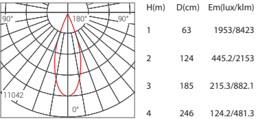
Beam Angle 38° 40W 3000K
